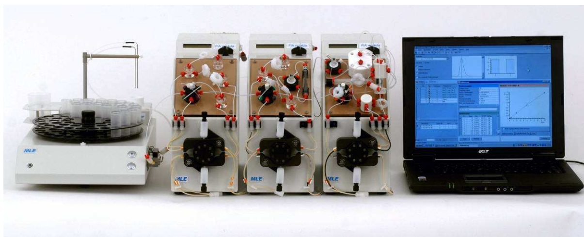
FIAmodula-3-Channel-System (here: ortho-Phosphat, Nitrat, Phenol-Index)
